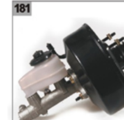
181 \Phi 23.81 XL No. XL036ZLB OEM 44610-38010.6.J02094/47201-38010
