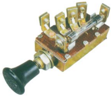
Head lamp switch Jk108 3p
